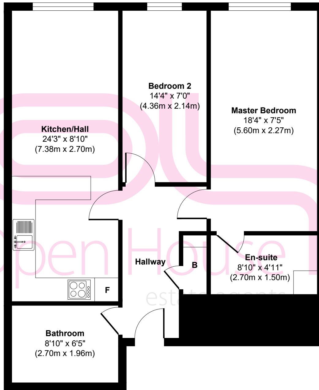
Floor Plan Approx. Gross Internal Floor Area 725 sq. ft / 67.38 sq. m
